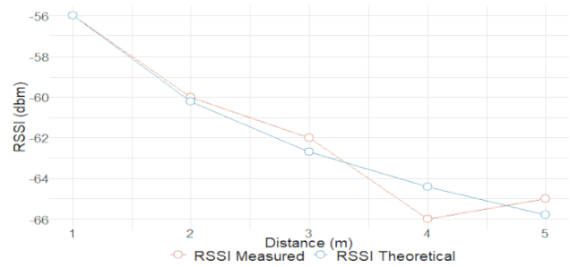
Figure 5. RSSI signal behavior in an unobstructed scenario
